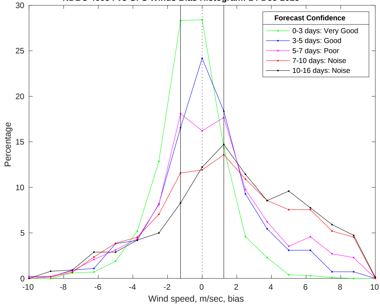
NDBC 46054 vs GFS Winds Bias Histogram: 14-Dec-2025
