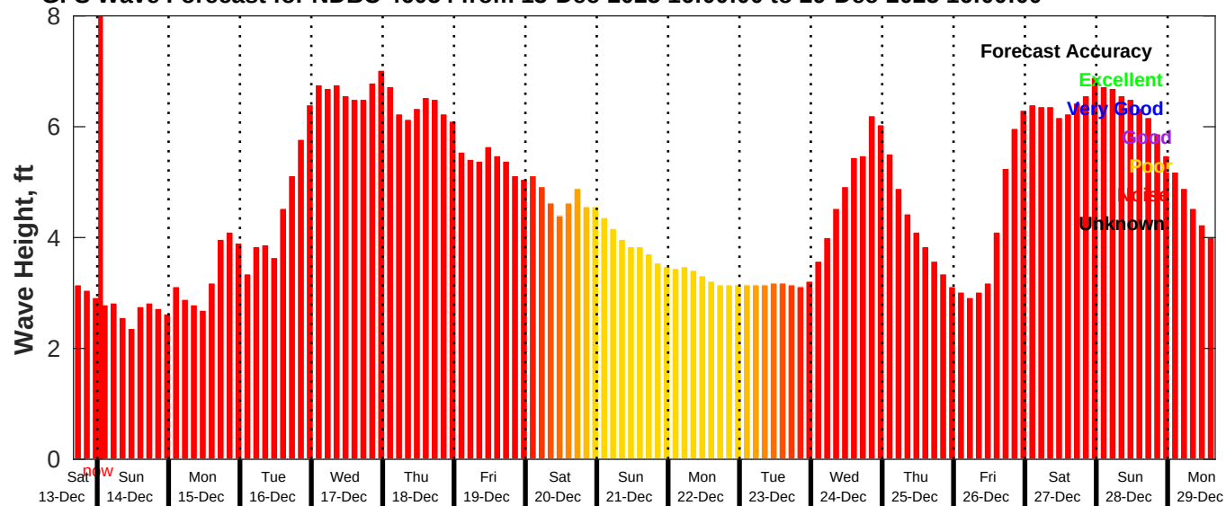
GFS Wave Forecast for NDBC 46054 from 13-Dec-2025 16:00:00 to 29-Dec-2025 16:00:00
