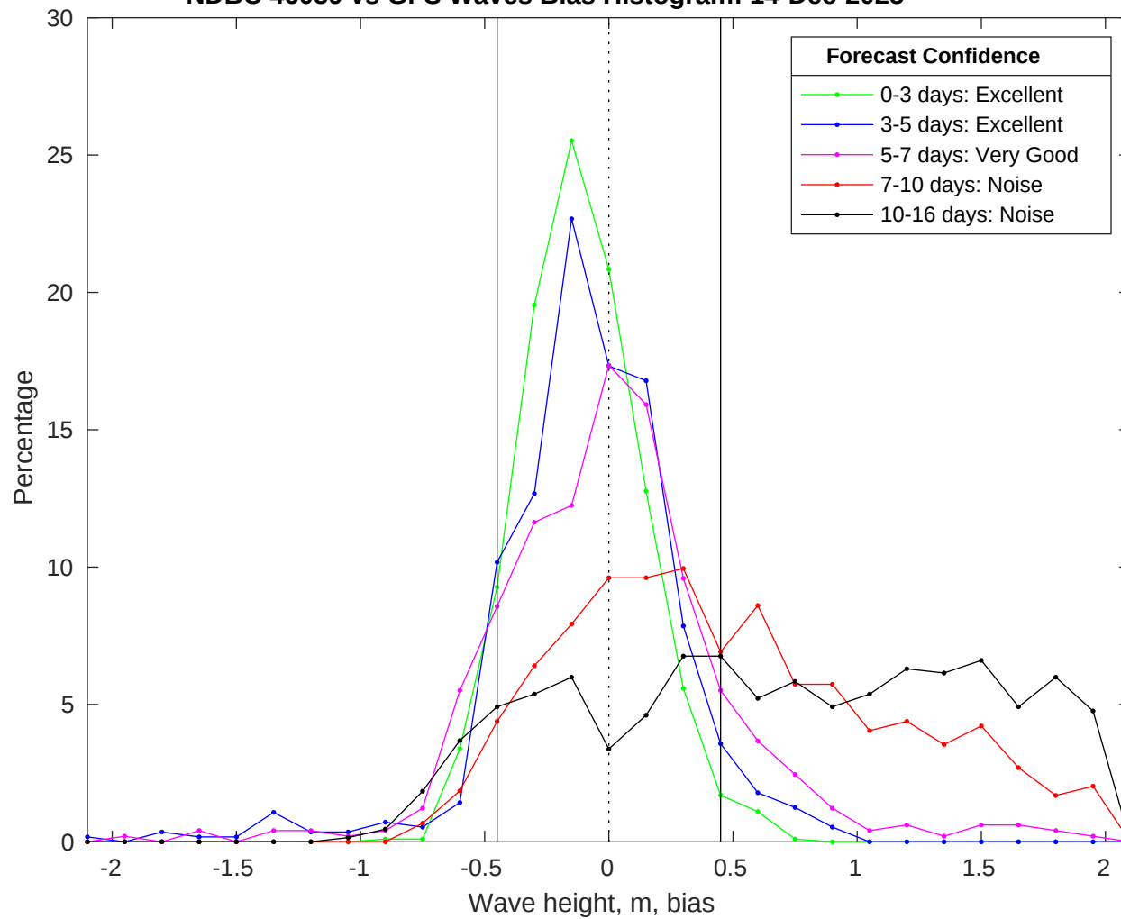
NDBC 46059 vs GFS Waves Bias Histogram: 14-Dec-2025
