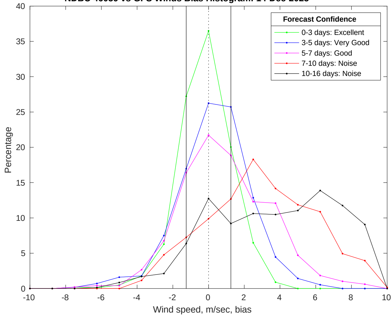
NDBC 46059 vs GFS Winds Bias Histogram: 14-Dec-2025
