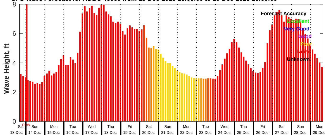
GFS Wave Forecast for NDBC 46069 from 13-Dec-2025 16:00:00 to 29-Dec-2025 16:00:00
