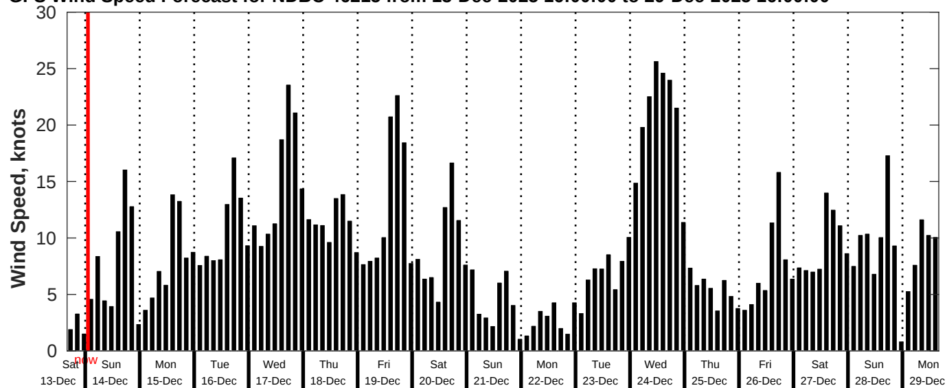
GFS Wind Speed Forecast for NDBC 46215 from 13-Dec-2025 16:00:00 to 29-Dec-2025 16:00:00
