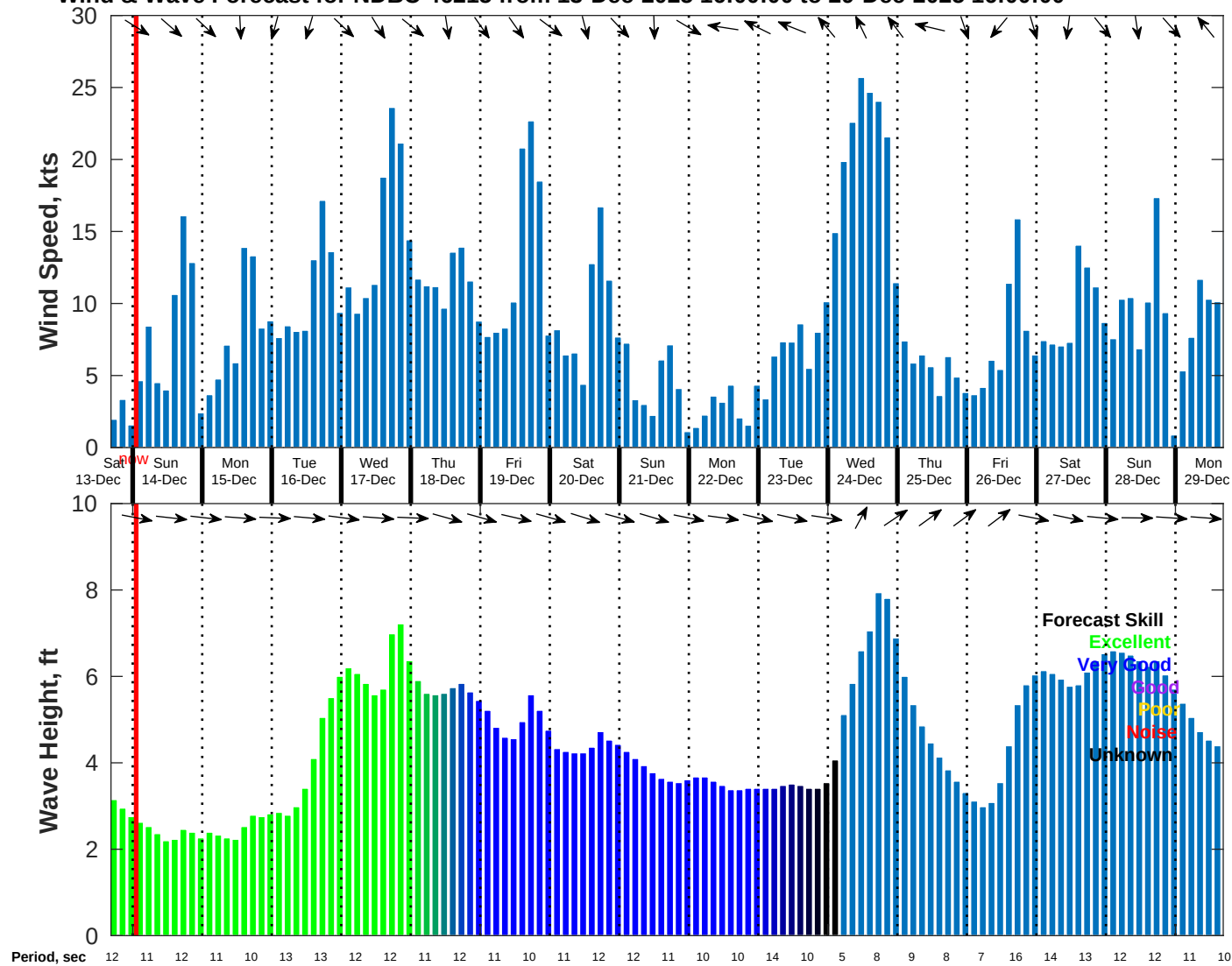
Wind & Wave Forecast for NDBC 46215 from 13-Dec-2025 16:00:00 to 29-Dec-2025 16:00:00
