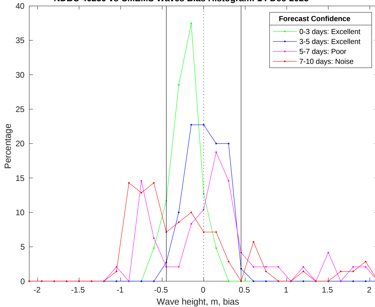
NDBC 46259 vs CMEMS Waves Bias Histogram: 14-Dec-2025
