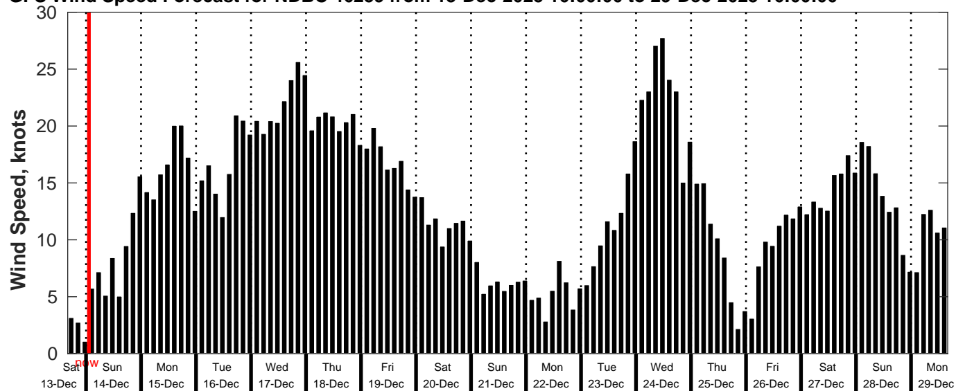
GFS Wind Speed Forecast for NDBC 46259 from 13-Dec-2025 16:00:00 to 29-Dec-2025 16:00:00
