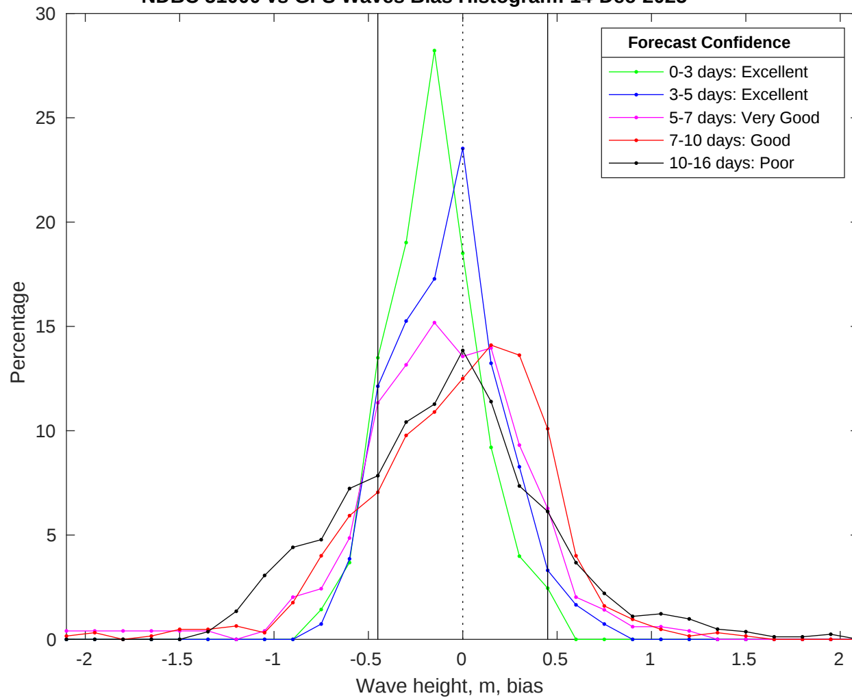
NDBC 51000 vs GFS Waves Bias Histogram: 14-Dec-2025
