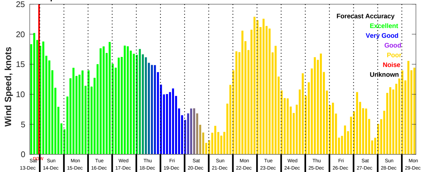
GFS Wind Speed Forecast for NDBC 51000 from 13-Dec-2025 14:00:00 to 29-Dec-2025 14:00:00
