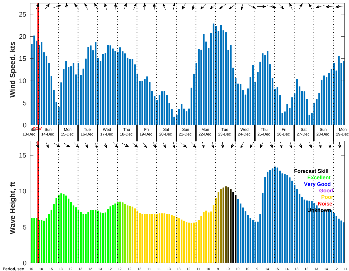
Wind & Wave Forecast for NDBC 51000 from 13-Dec-2025 14:00:00 to 29-Dec-2025 14:00:00
