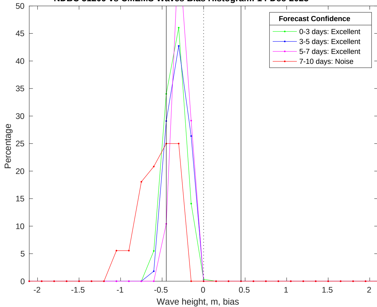
NDBC 51209 vs CMEMS Waves Bias Histogram: 14-Dec-2025
