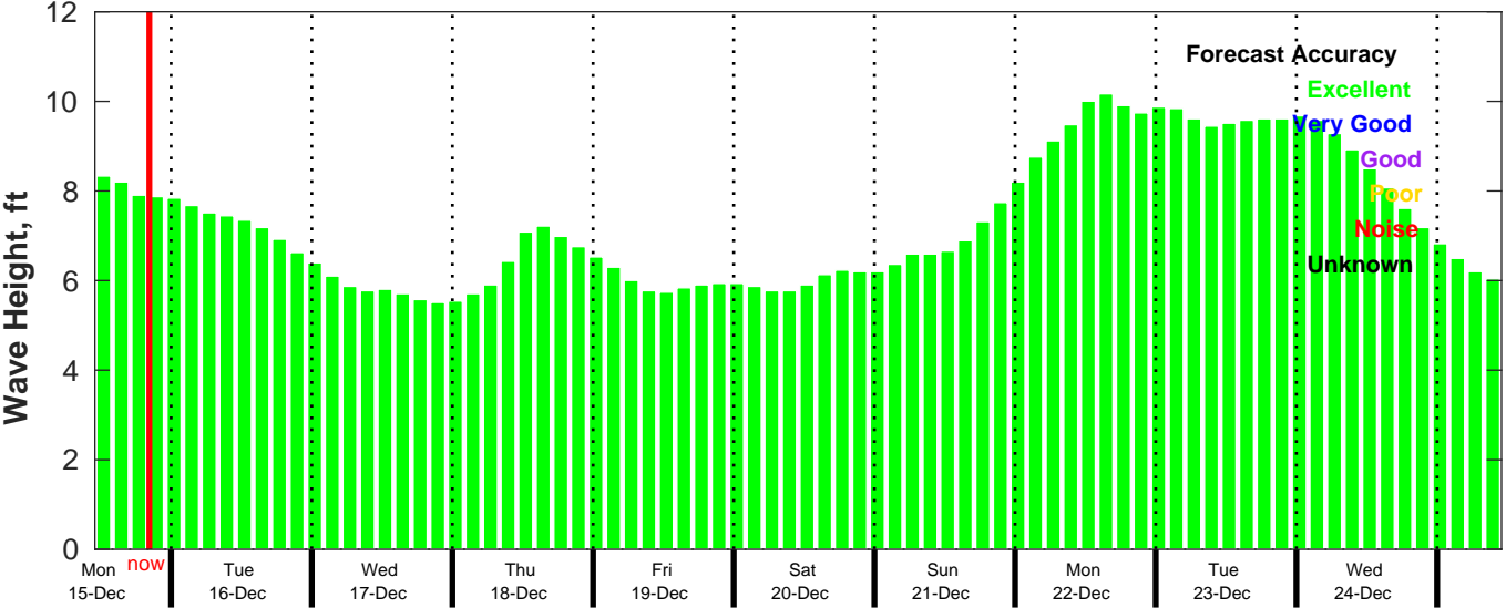
CMEMS Wave Forecast for NDBC 52211 from 14-Dec-2025 11:00:00 to 24-Dec-2025 11:00:00
