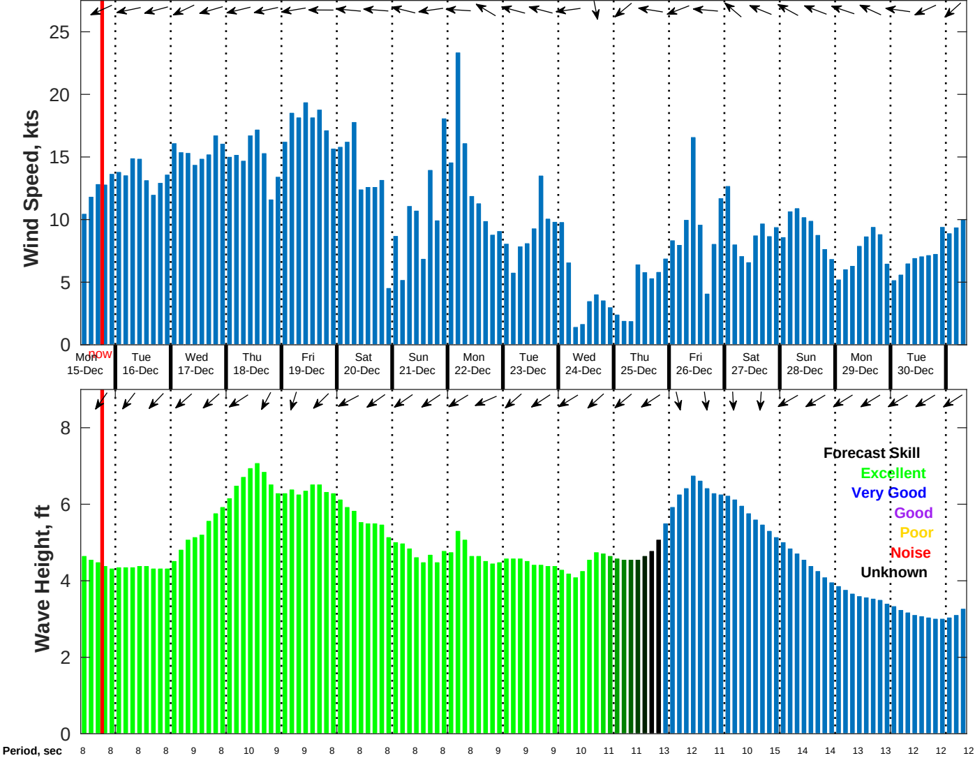
Wind & Wave Forecast for NDBC 52212 from 14-Dec-2025 09:00:00 to 30-Dec-2025 09:00:00
