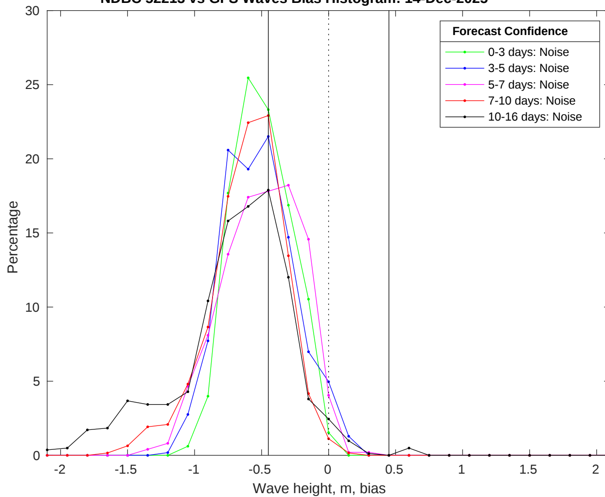
NDBC 52213 vs GFS Waves Bias Histogram: 14-Dec-2025
