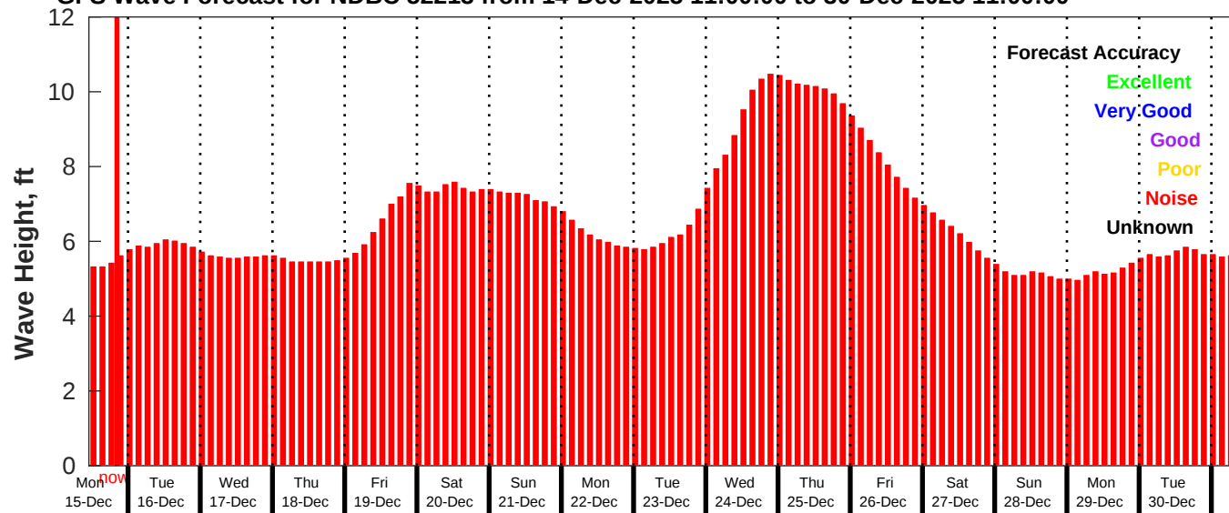
GFS Wave Forecast for NDBC 52213 from 14-Dec-2025 11:00:00 to 30-Dec-2025 11:00:00
