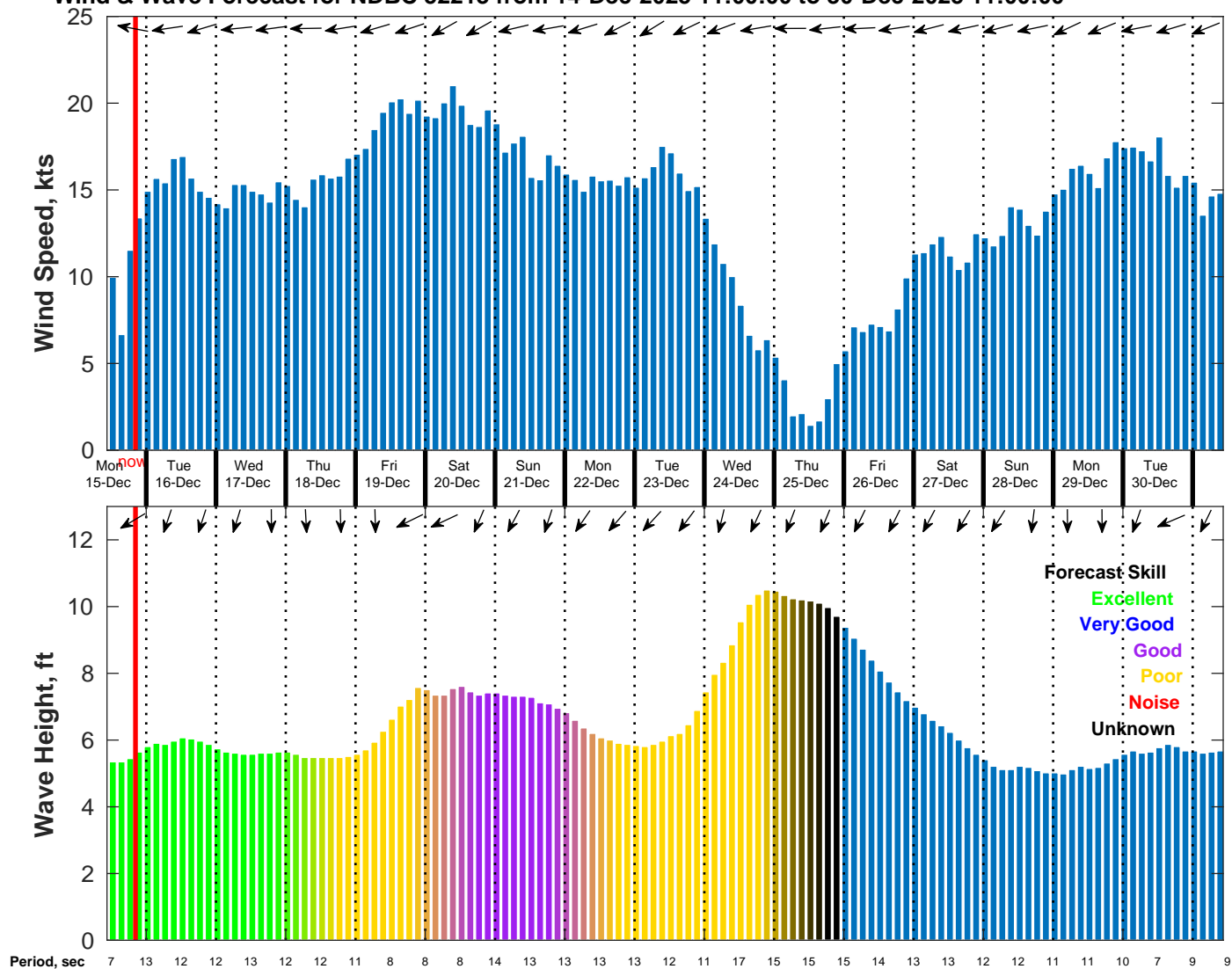
Wind & Wave Forecast for NDBC 52213 from 14-Dec-2025 11:00:00 to 30-Dec-2025 11:00:00
