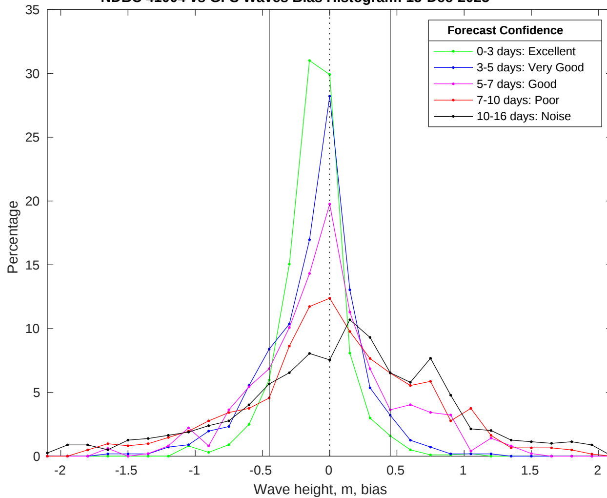
NDBC 41004 vs GFS Waves Bias Histogram: 15-Dec-2025
