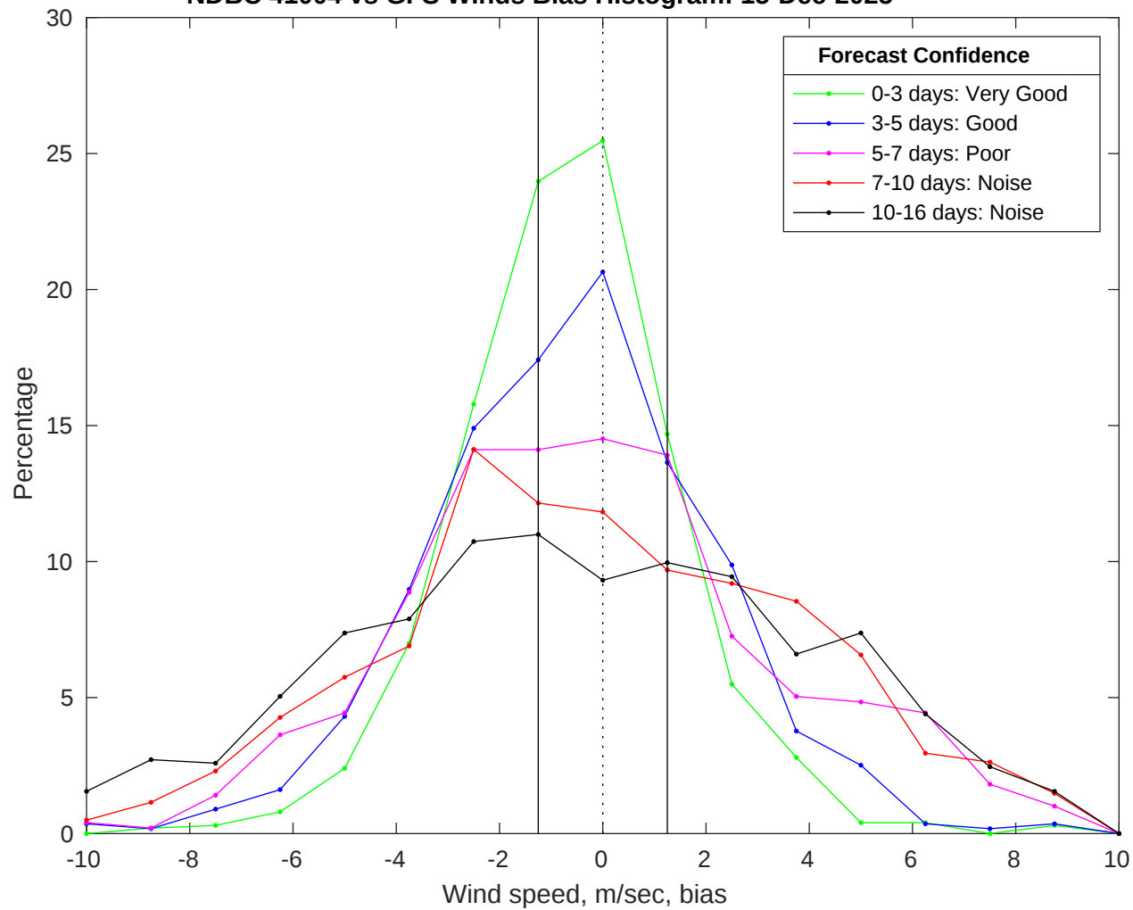
NDBC 41004 vs GFS Winds Bias Histogram: 15-Dec-2025
