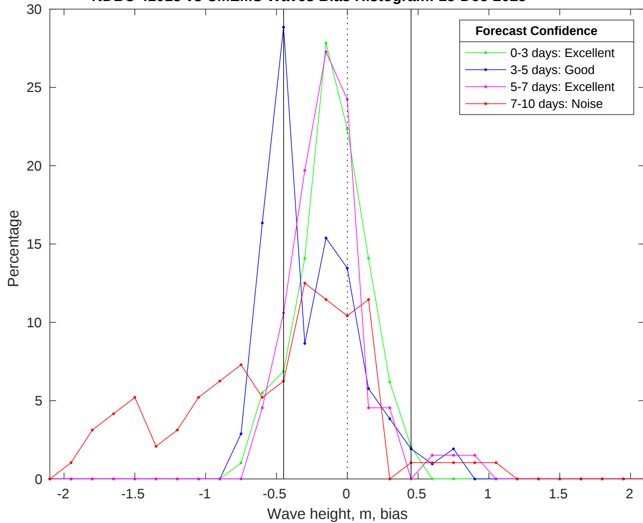
NDBC 41013 vs CMEMS Waves Bias Histogram: 15-Dec-2025
