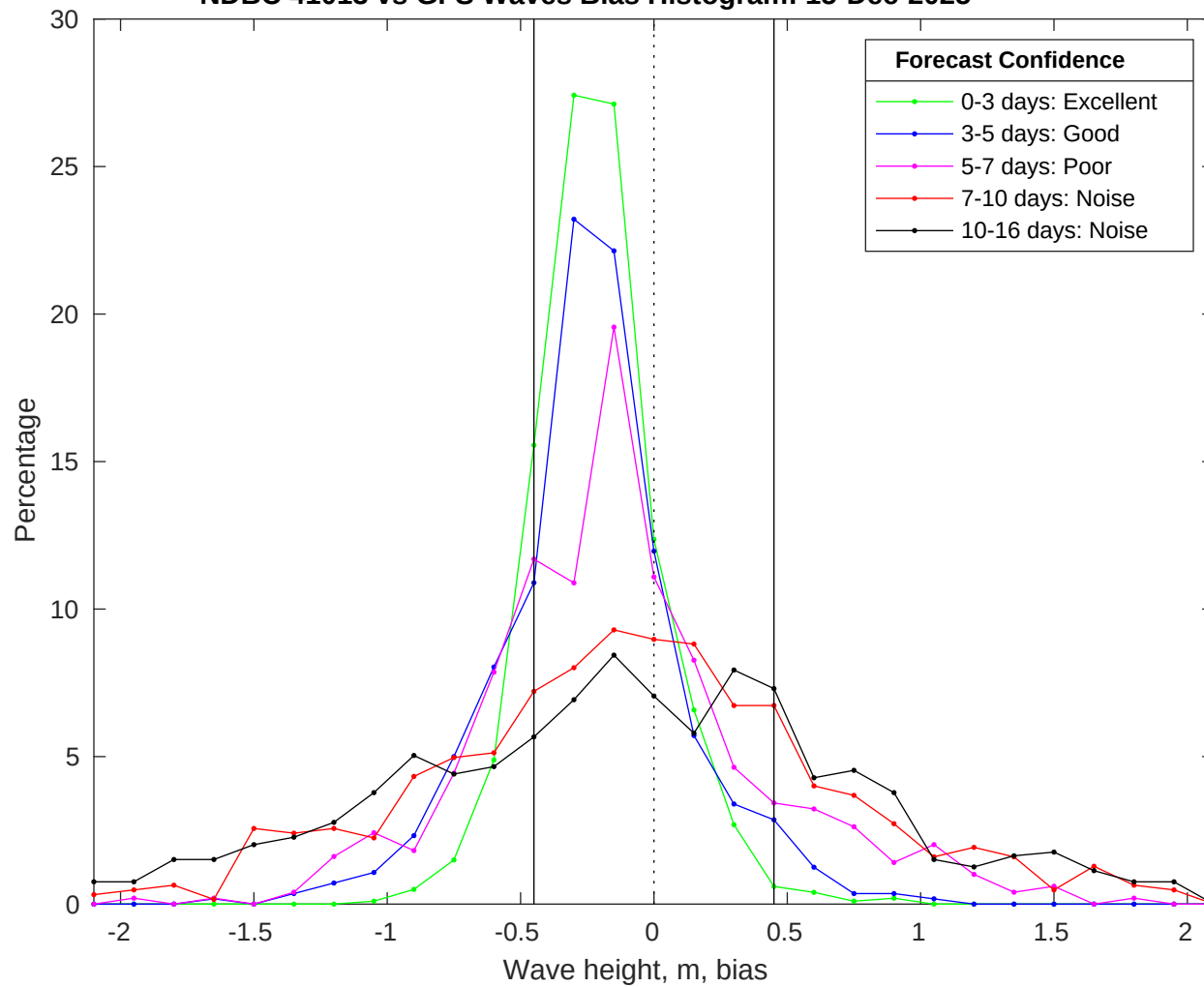
NDBC 41013 vs GFS Waves Bias Histogram: 15-Dec-2025
