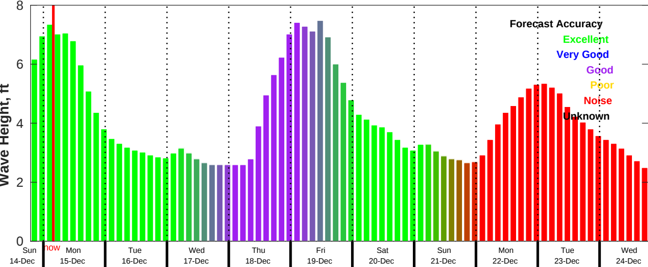
CMEMS Wave Forecast for NDBC 41013 from 14-Dec-2025 19:00:00 to 24-Dec-2025 19:00:00
