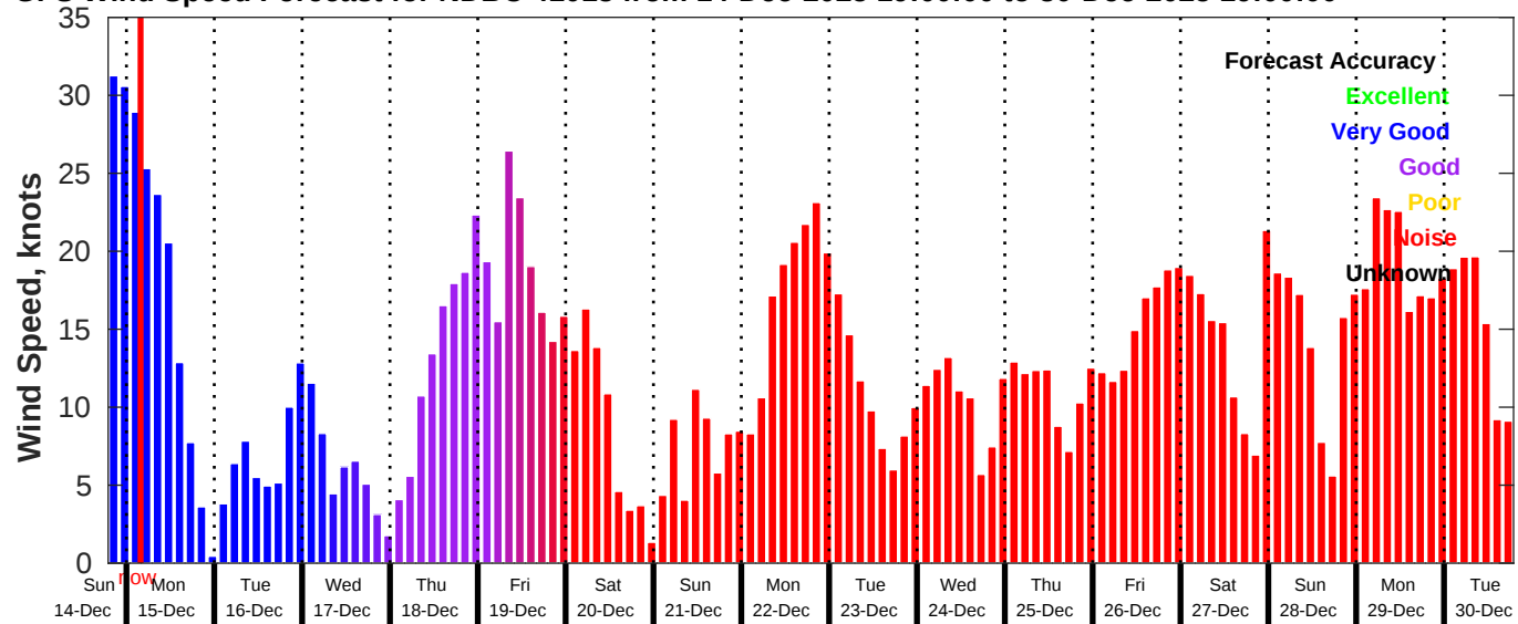
GFS Wind Speed Forecast for NDBC 41013 from 14-Dec-2025 19:00:00 to 30-Dec-2025 19:00:00
