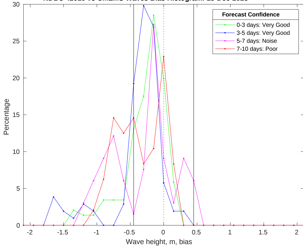
NDBC 42019 vs CMEMS Waves Bias Histogram: 15-Dec-2025
