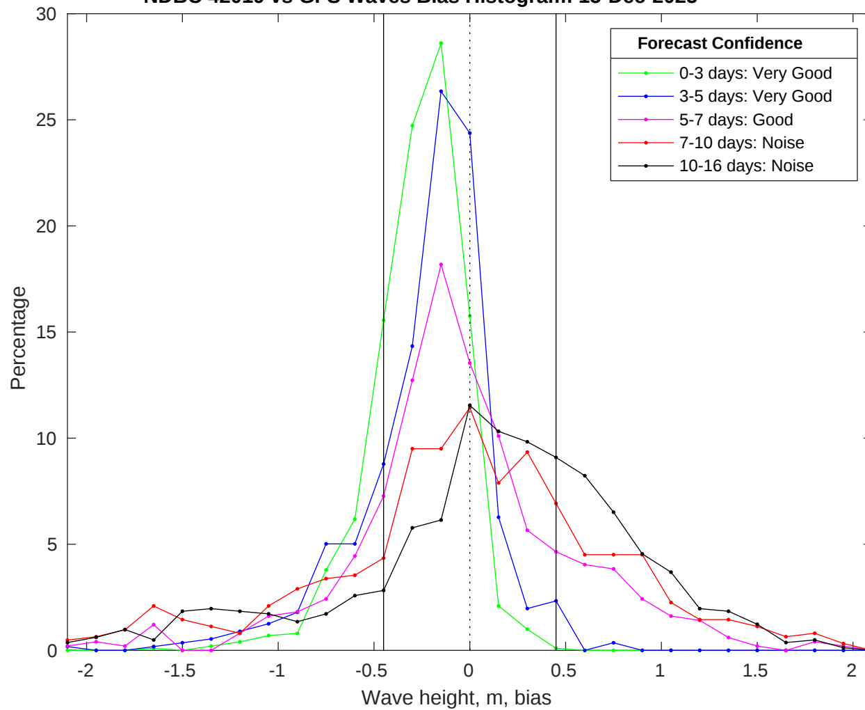
NDBC 42019 vs GFS Waves Bias Histogram: 15-Dec-2025
