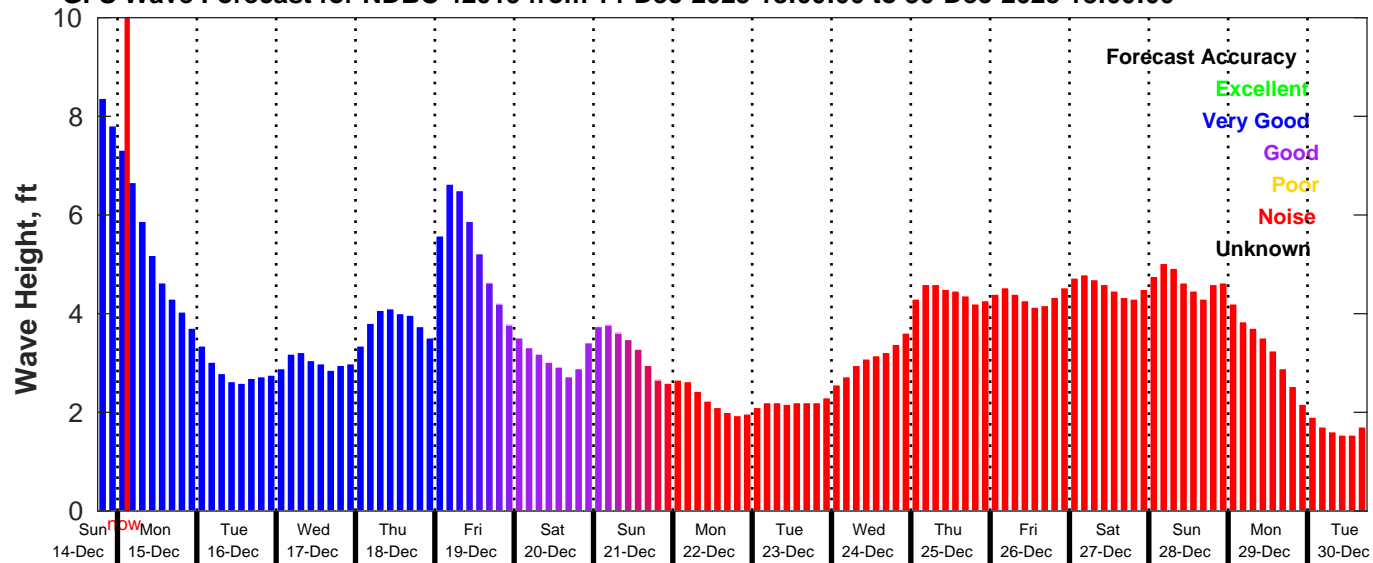
GFS Wave Forecast for NDBC 42019 from 14-Dec-2025 18:00:00 to 30-Dec-2025 18:00:00
