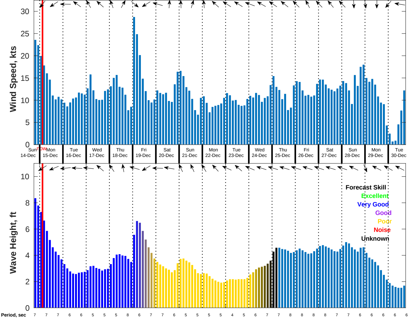
Wind & Wave Forecast for NDBC 42019 from 14-Dec-2025 18:00:00 to 30-Dec-2025 18:00:00
