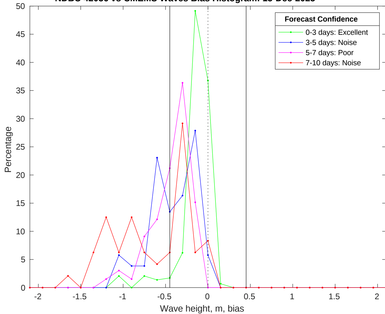
NDBC 42036 vs CMEMS Waves Bias Histogram: 15-Dec-2025
