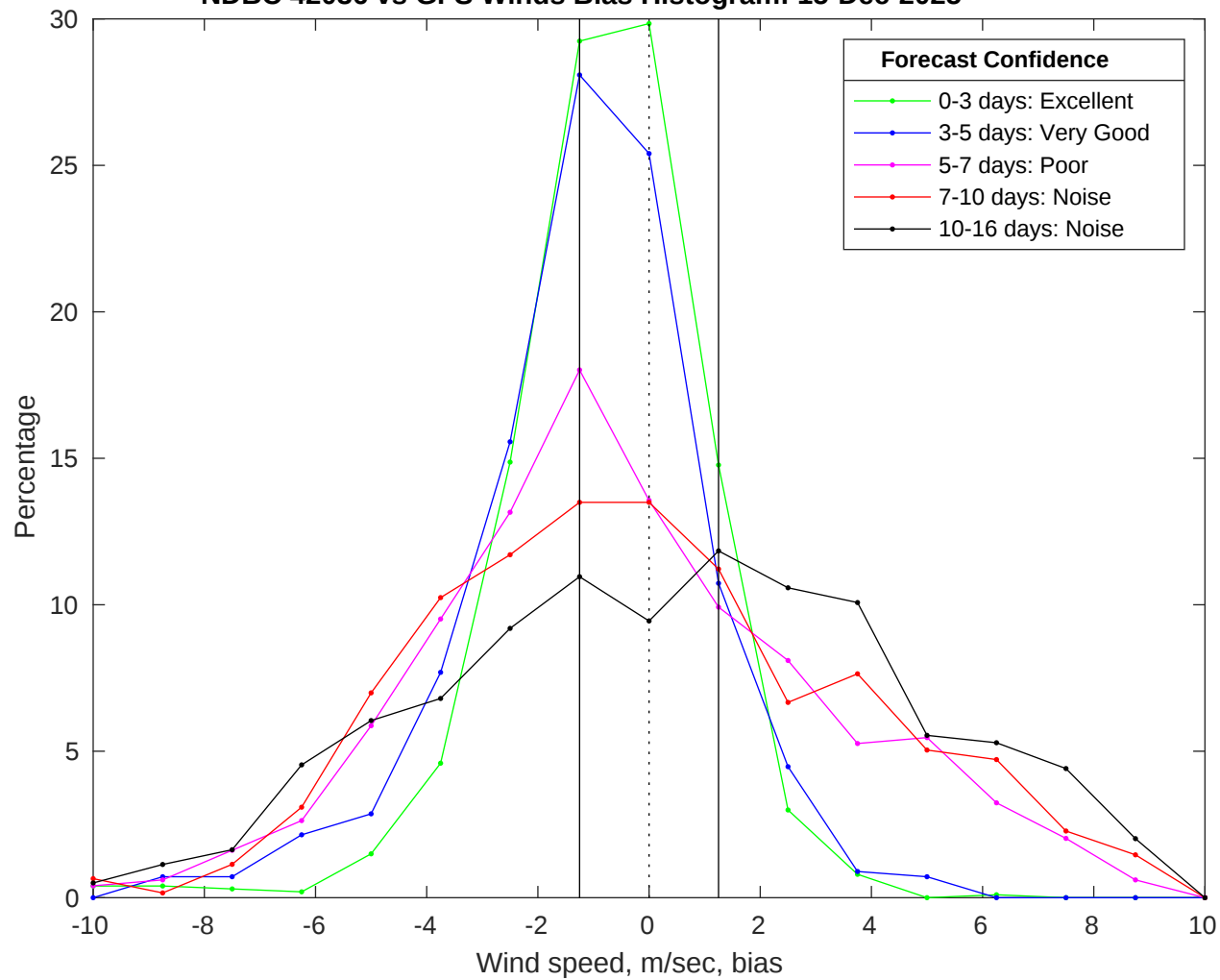
NDBC 42036 vs GFS Winds Bias Histogram: 15-Dec-2025
