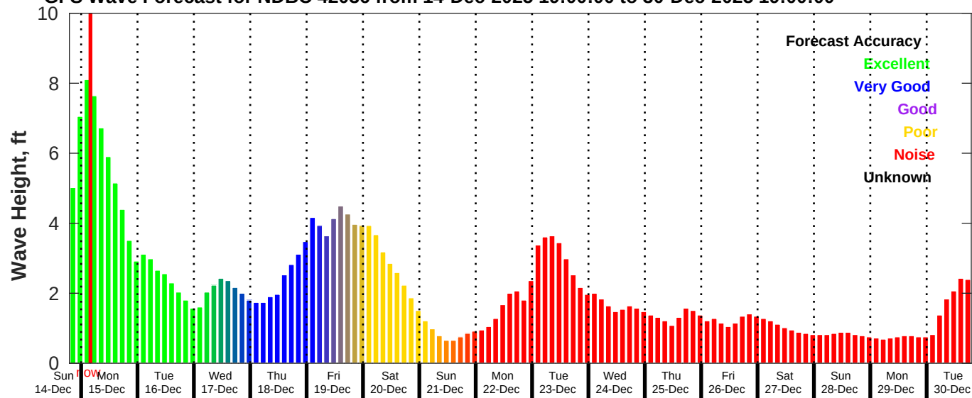
GFS Wave Forecast for NDBC 42036 from 14-Dec-2025 19:00:00 to 30-Dec-2025 19:00:00
