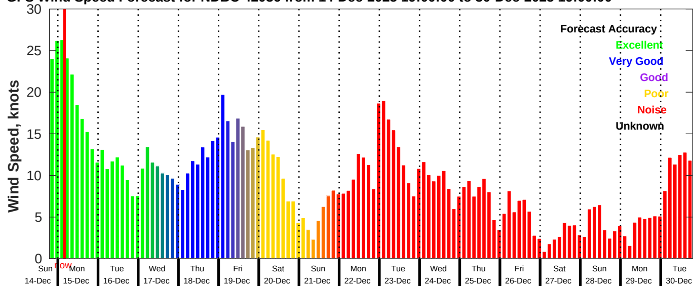
GFS Wind Speed Forecast for NDBC 42036 from 14-Dec-2025 19:00:00 to 30-Dec-2025 19:00:00
