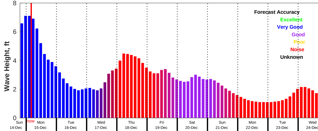
CMEMS Wave Forecast for NDBC 42040 from 14-Dec-2025 19:00:00 to 24-Dec-2025 19:00:00
