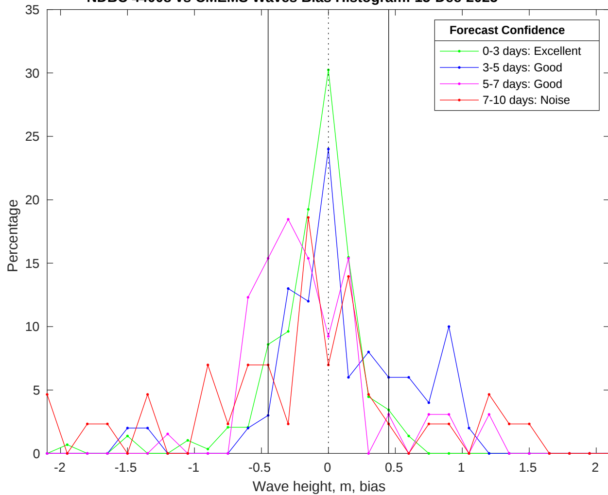
NDBC 44008 vs CMEMS Waves Bias Histogram: 15-Dec-2025
