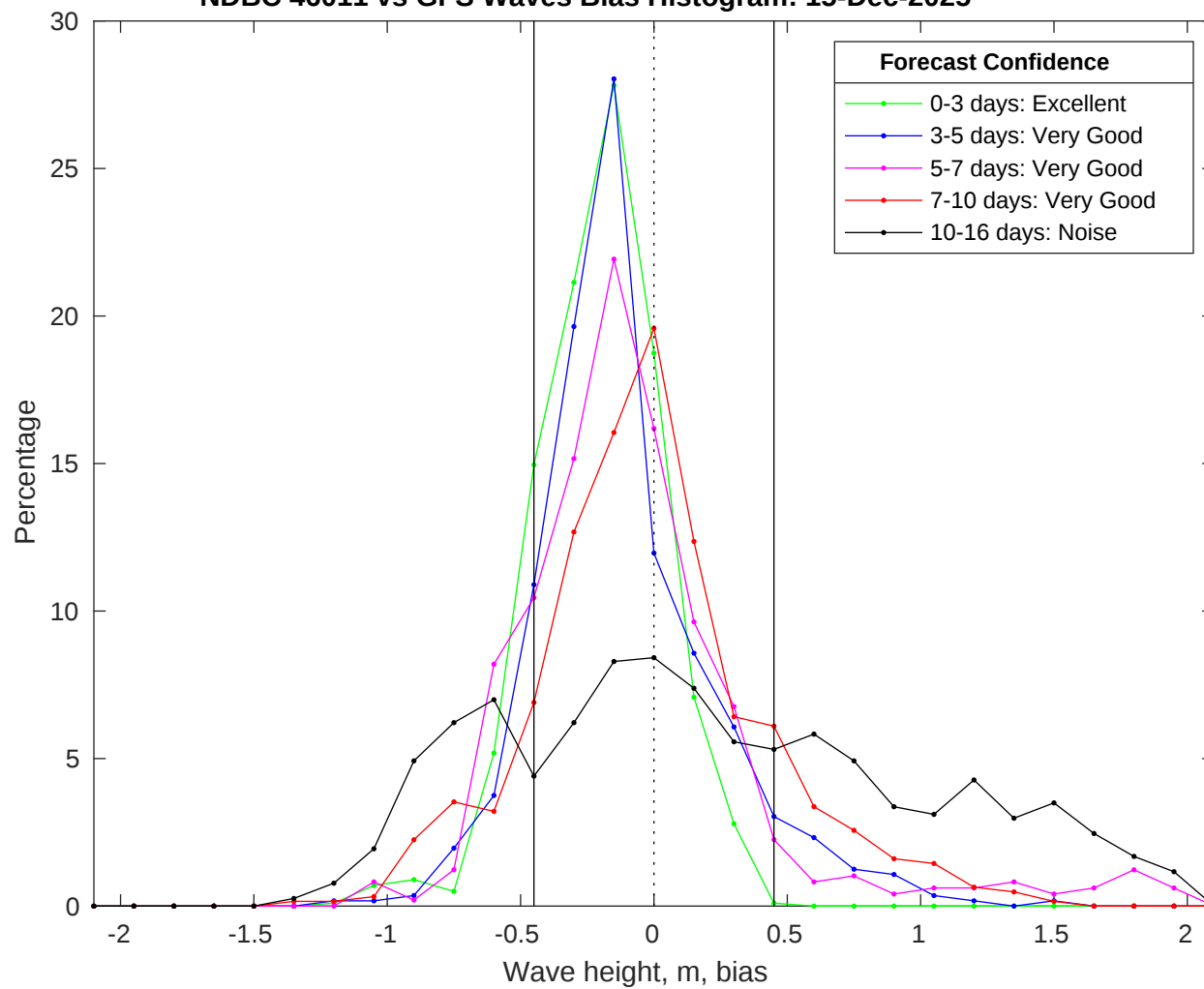
NDBC 46011 vs GFS Waves Bias Histogram: 15-Dec-2025
