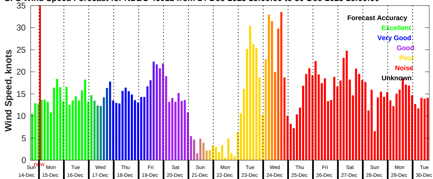
GFS Wind Speed Forecast for NDBC 46011 from 14-Dec-2025 16:00:00 to 30-Dec-2025 16:00:00
