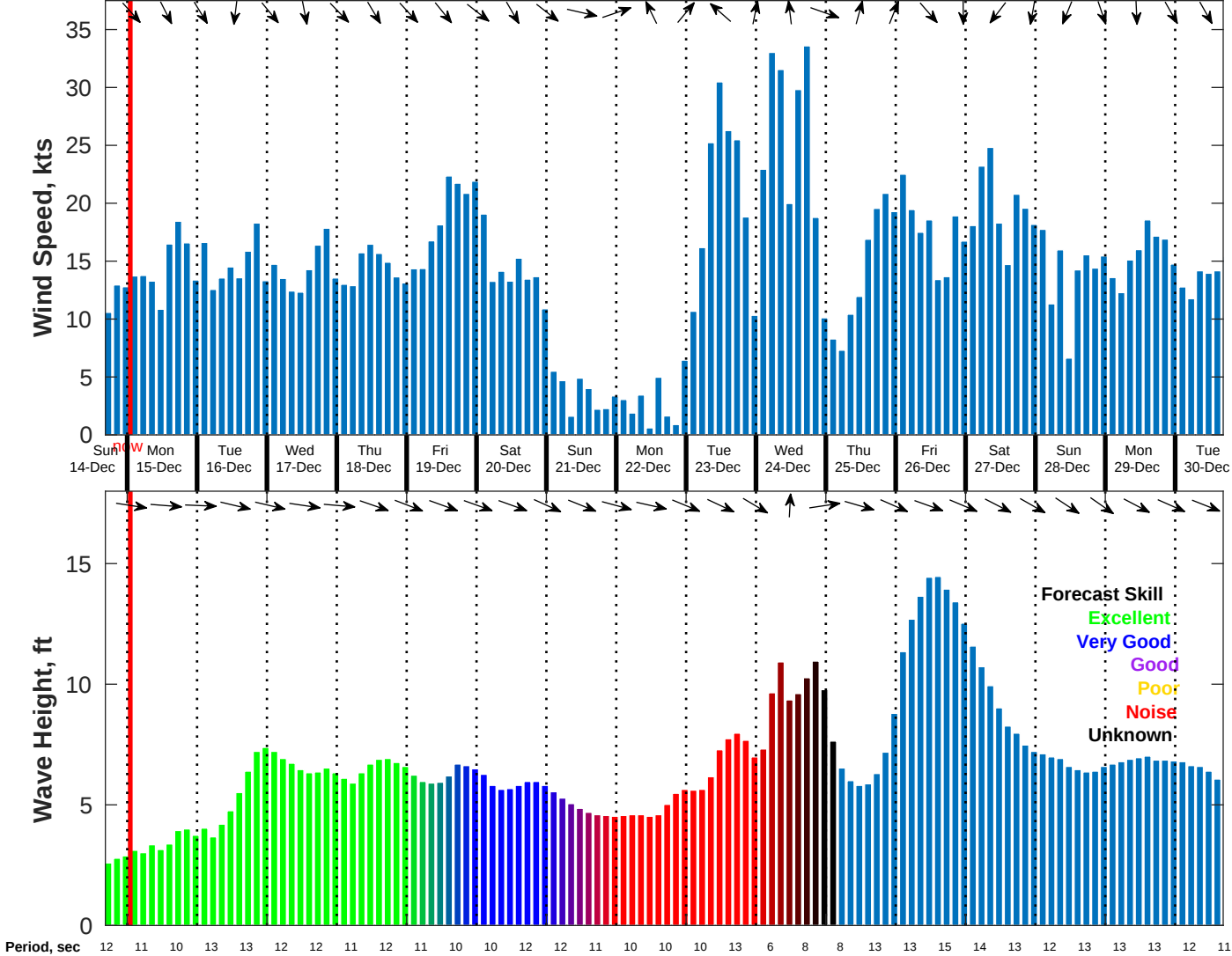
Wind & Wave Forecast for NDBC 46011 from 14-Dec-2025 16:00:00 to 30-Dec-2025 16:00:00
