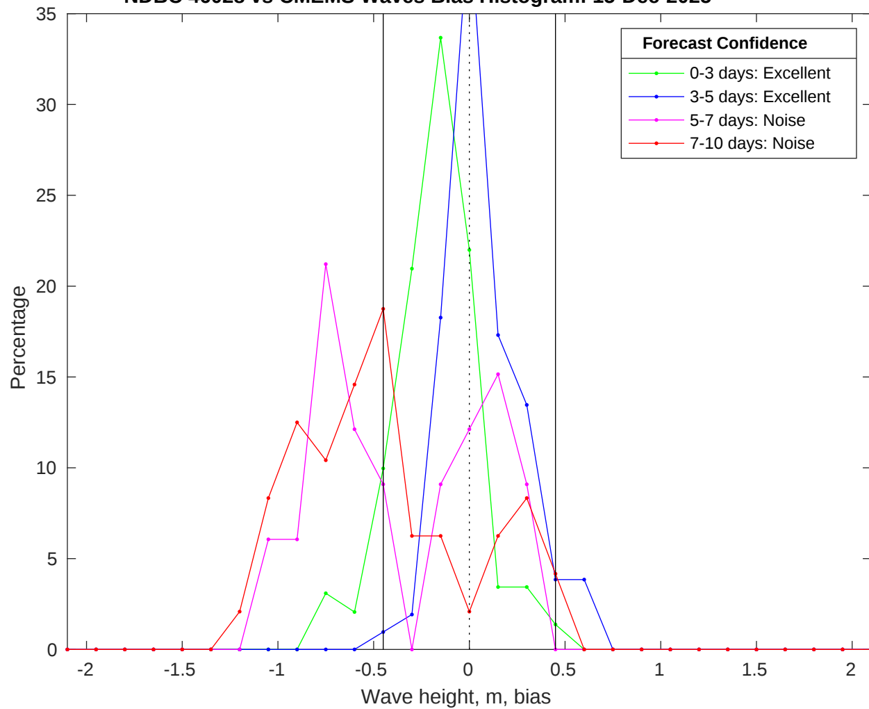
NDBC 46028 vs CMEMS Waves Bias Histogram: 15-Dec-2025
