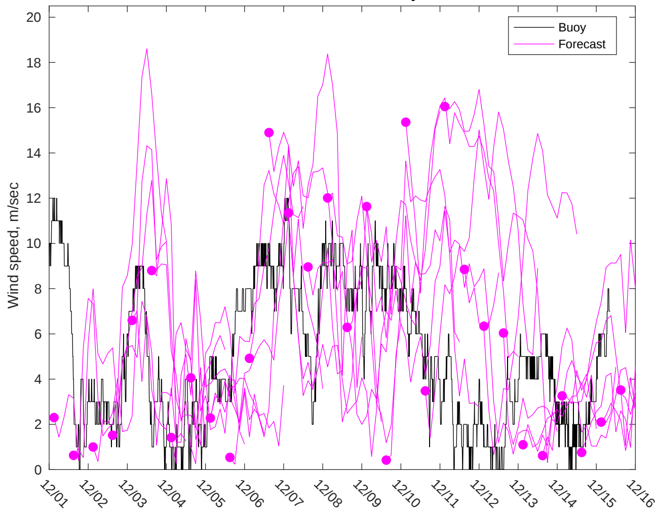
NDBC 46028 vs GFS Winds: 7 to 10 day forecast
