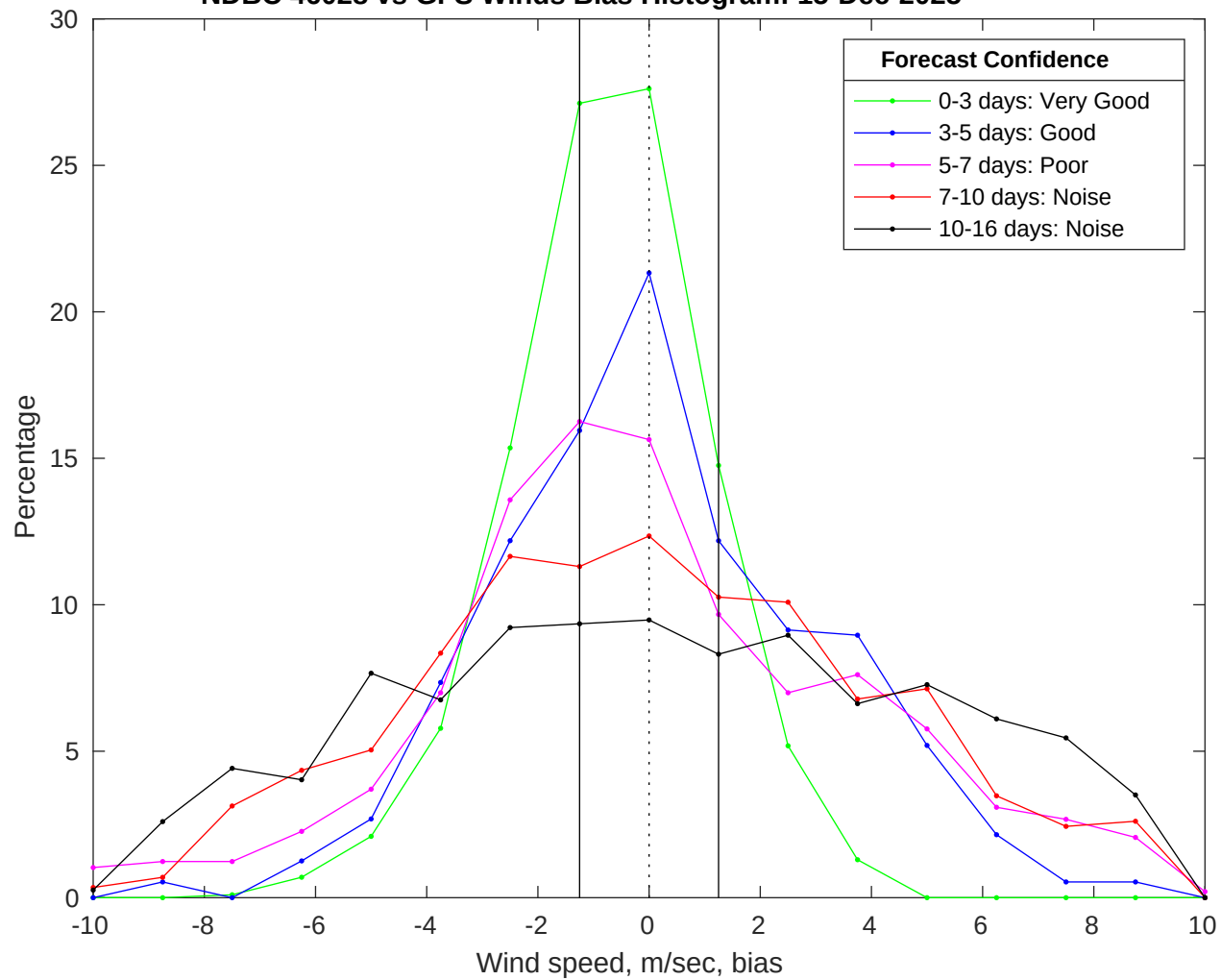
NDBC 46028 vs GFS Winds Bias Histogram: 15-Dec-2025
