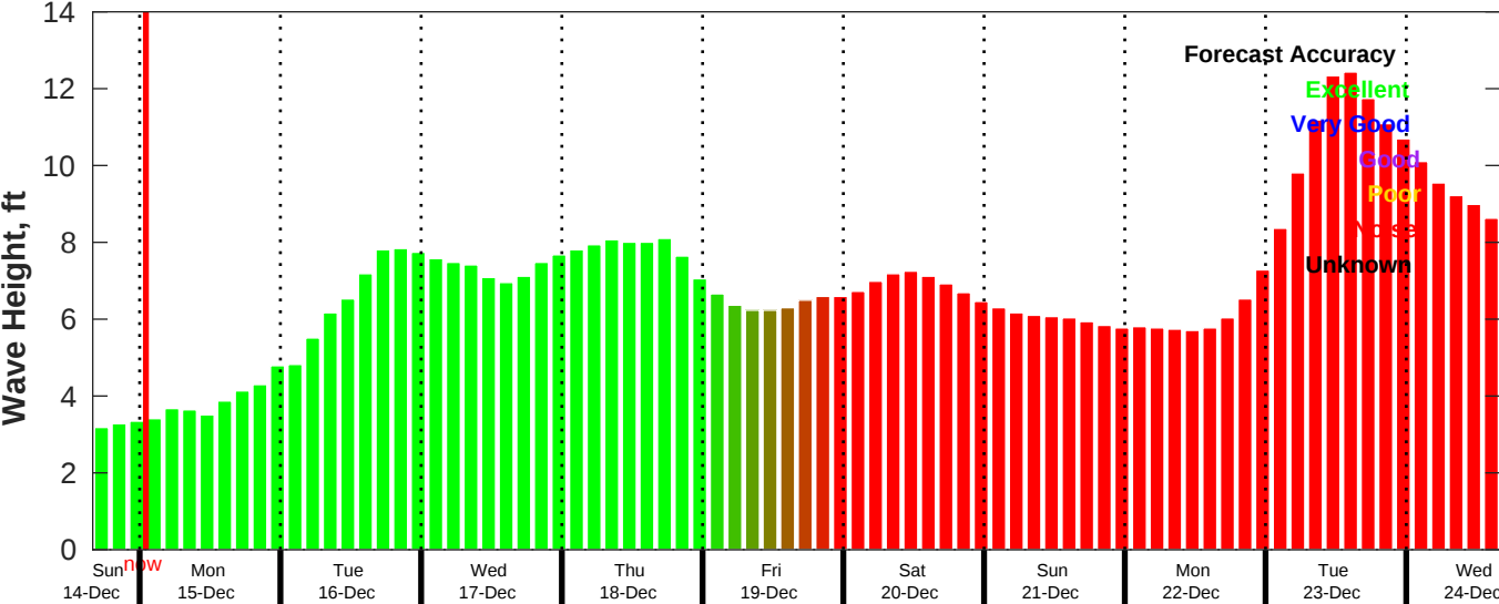
CMEMS Wave Forecast for NDBC 46028 from 14-Dec-2025 16:00:00 to 24-Dec-2025 16:00:00
