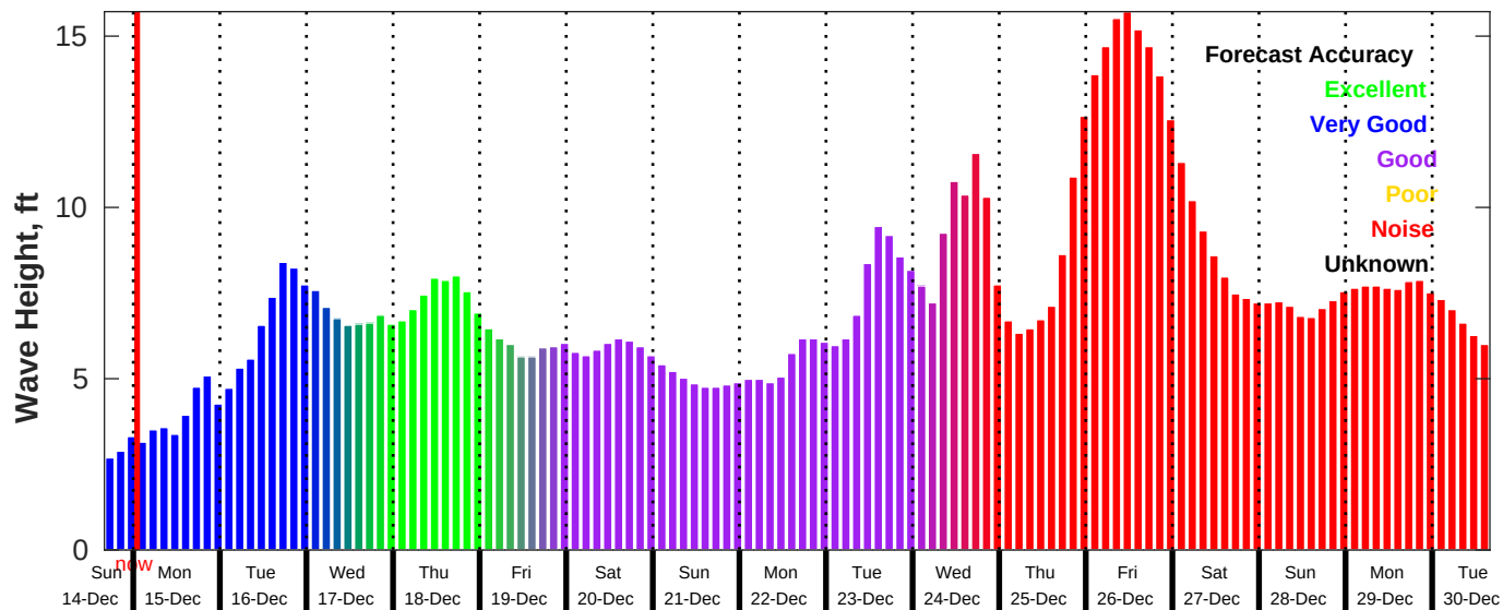
GFS Wave Forecast for NDBC 46028 from 14-Dec-2025 16:00:00 to 30-Dec-2025 16:00:00
