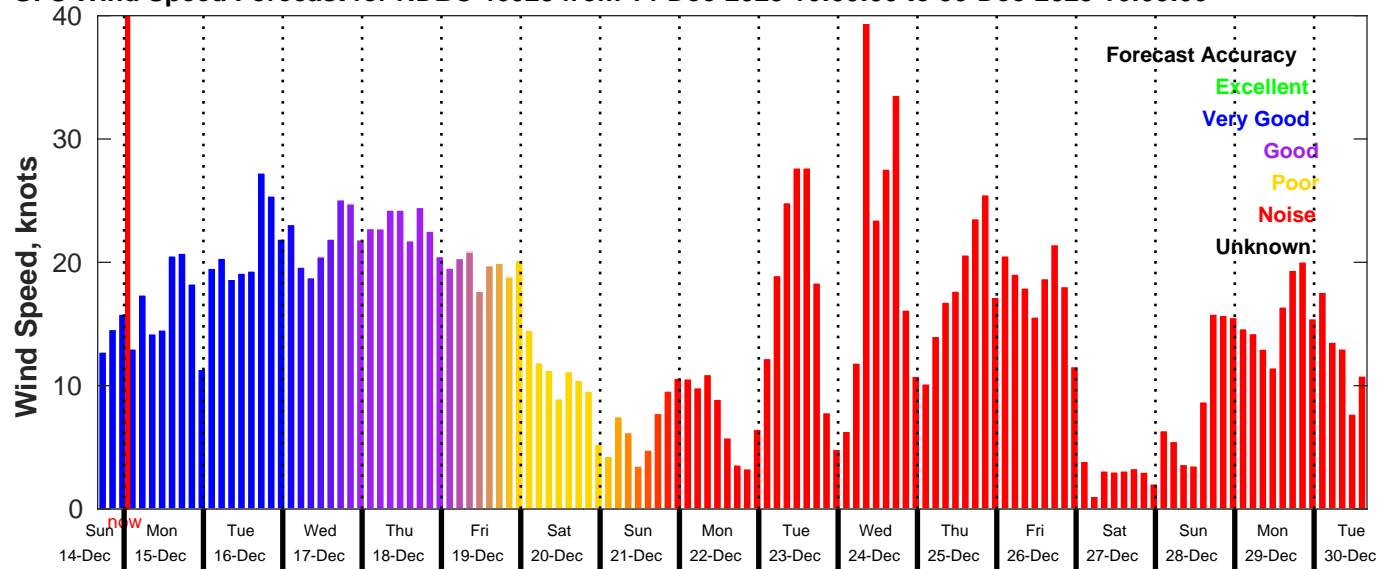
GFS Wind Speed Forecast for NDBC 46028 from 14-Dec-2025 16:00:00 to 30-Dec-2025 16:00:00
