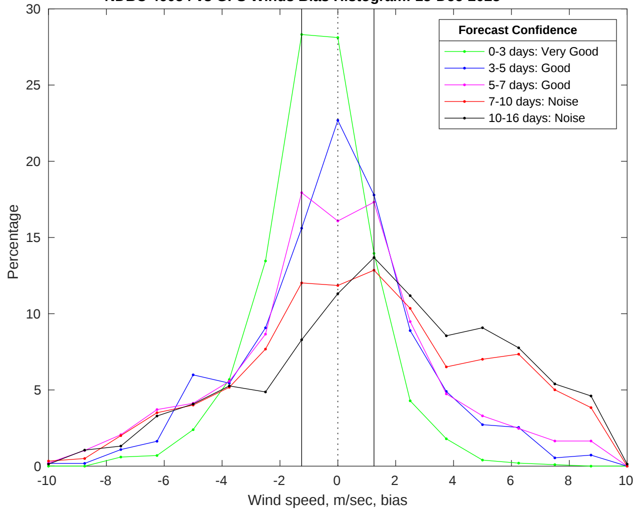
NDBC 46054 vs GFS Winds Bias Histogram: 15-Dec-2025
