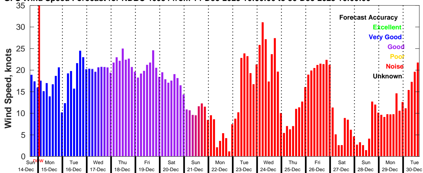
GFS Wind Speed Forecast for NDBC 46054 from 14-Dec-2025 16:00:00 to 30-Dec-2025 16:00:00
