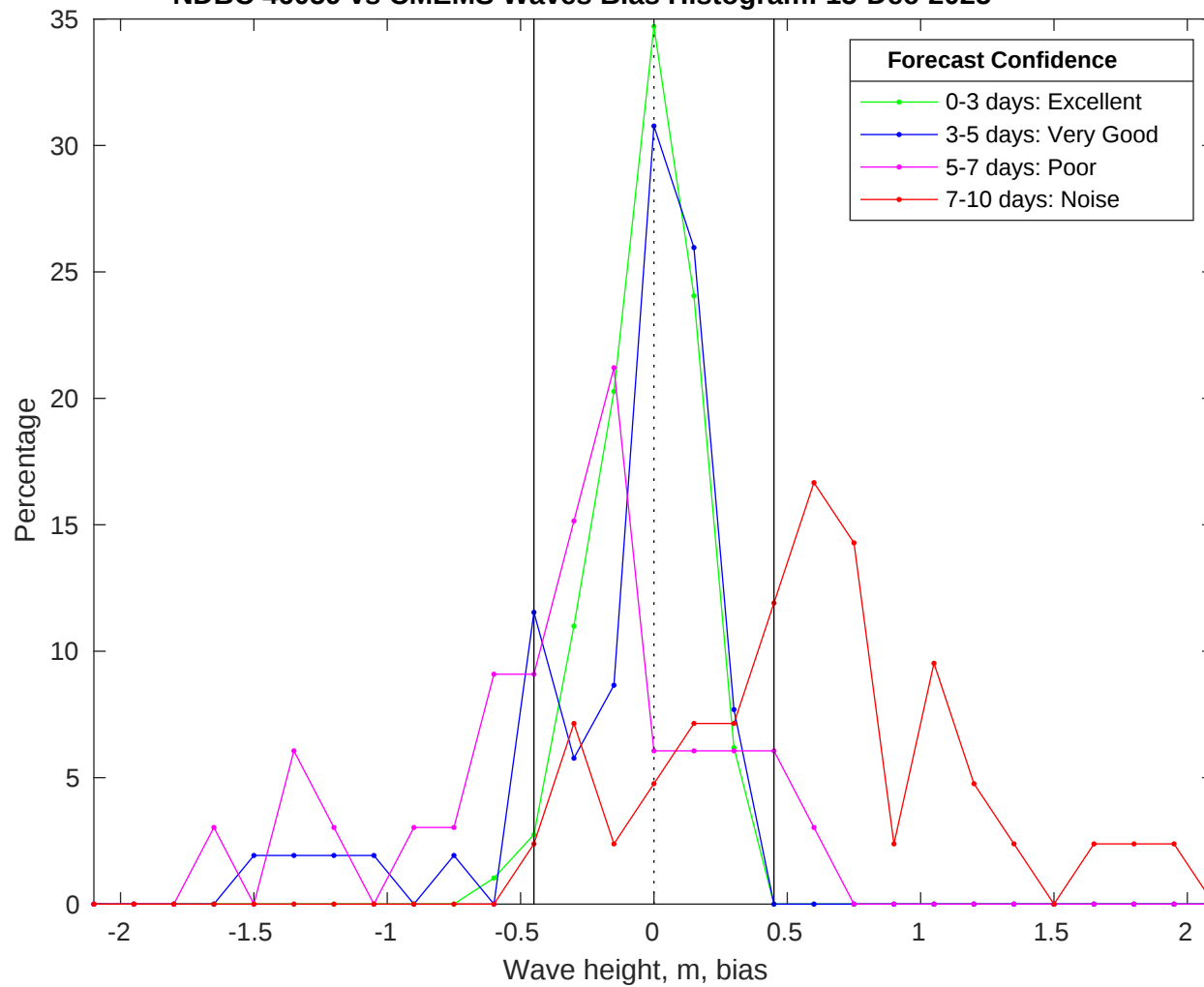
NDBC 46059 vs CMEMS Waves Bias Histogram: 15-Dec-2025
