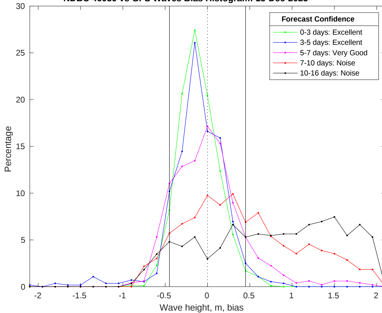
NDBC 46059 vs GFS Waves Bias Histogram: 15-Dec-2025
