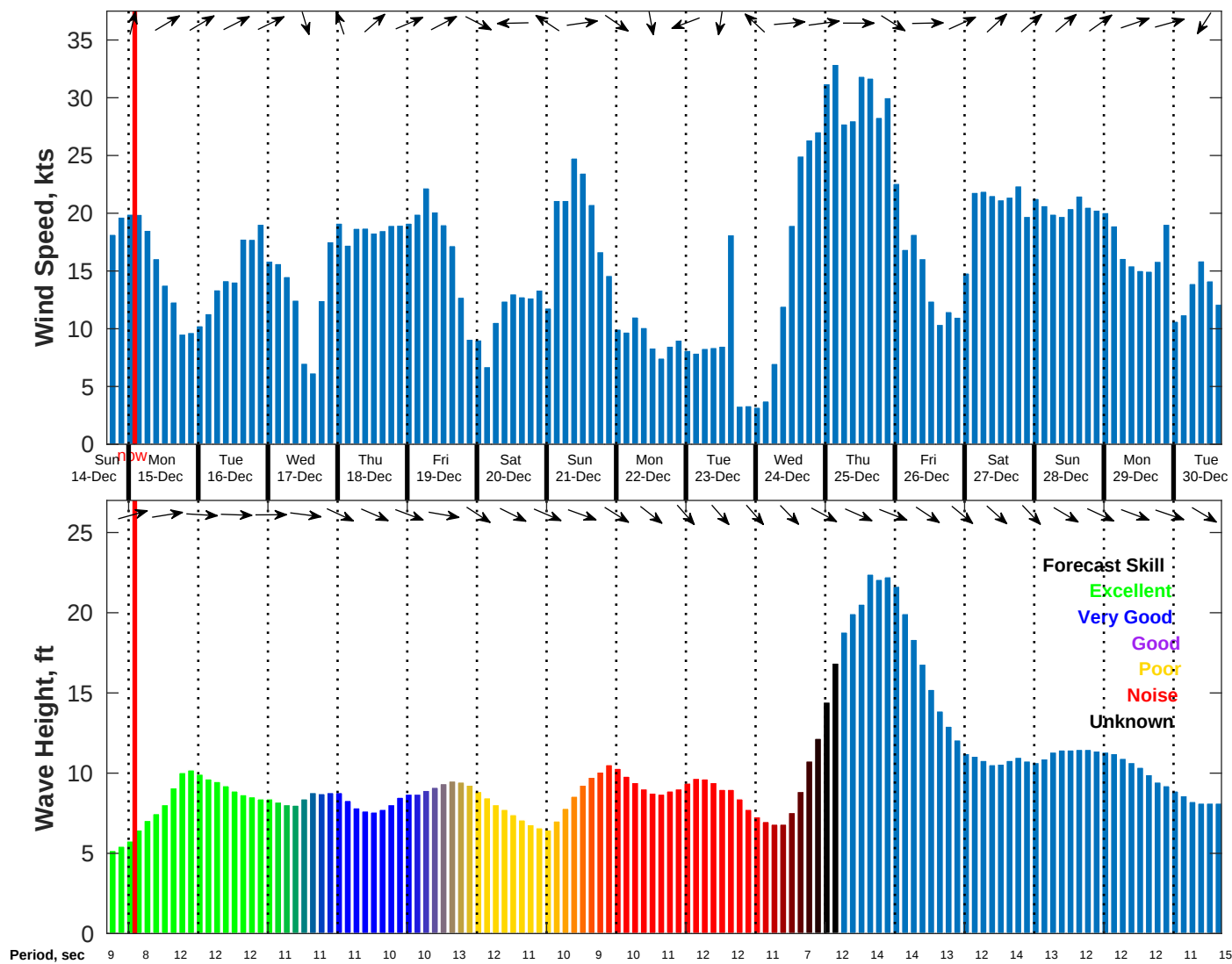
Wind & Wave Forecast for NDBC 46059 from 14-Dec-2025 17:00:00 to 30-Dec-2025 17:00:00
