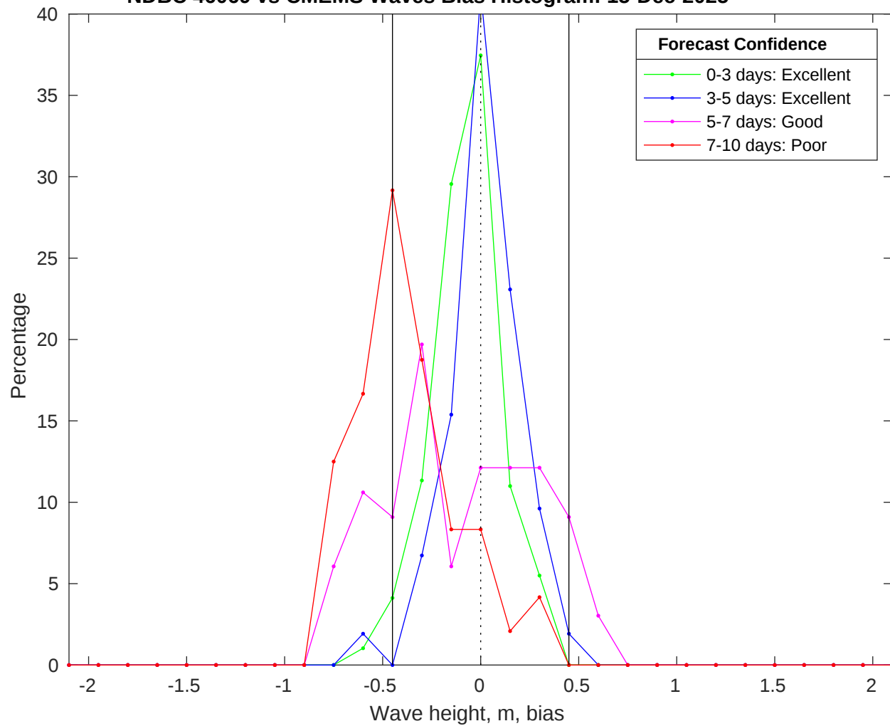
NDBC 46069 vs CMEMS Waves Bias Histogram: 15-Dec-2025
