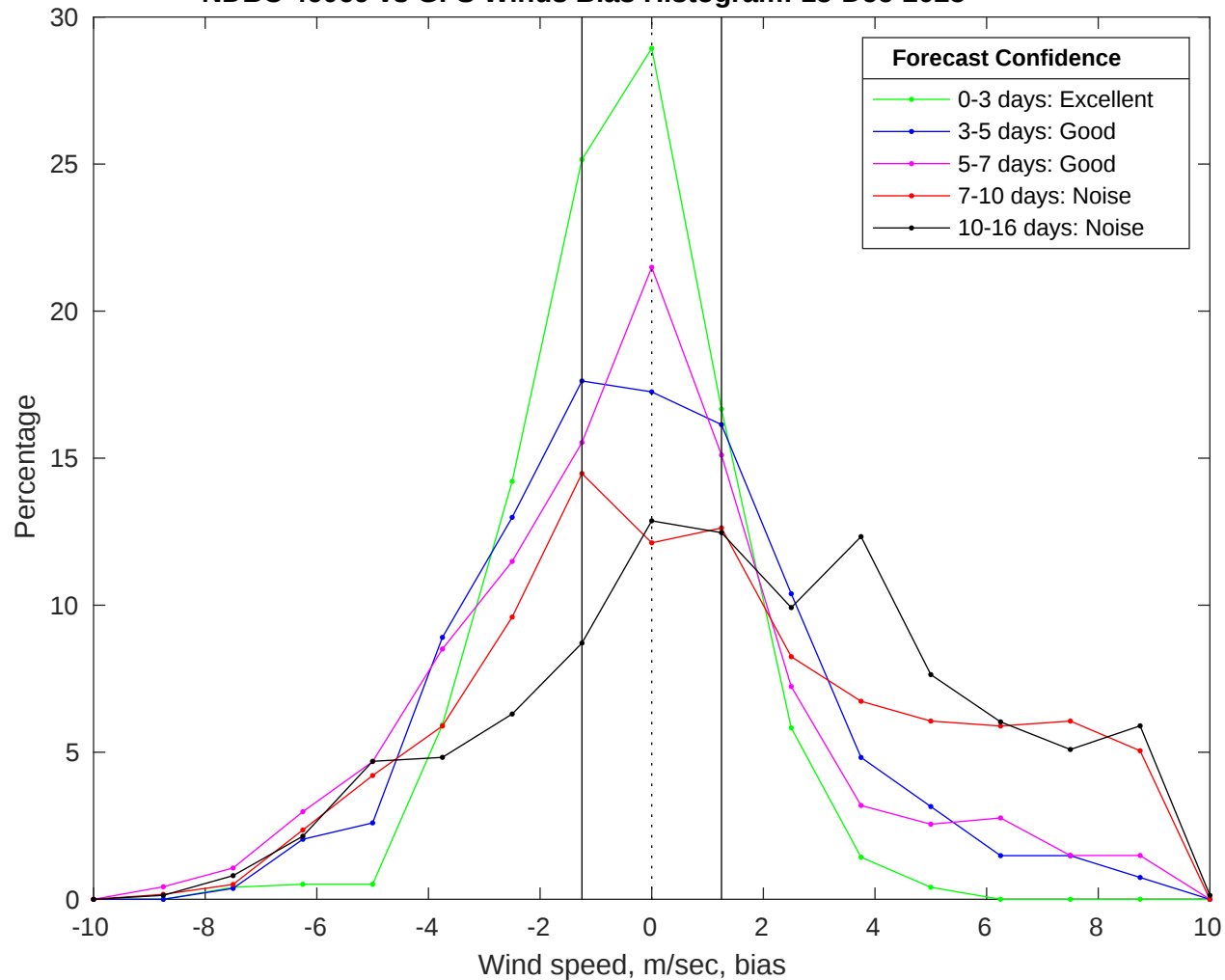
NDBC 46069 vs GFS Winds Bias Histogram: 15-Dec-2025
